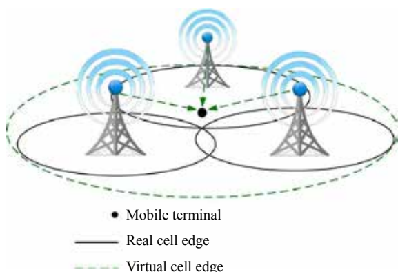
Figure 3: Multi-point coordinated cell zooming.
