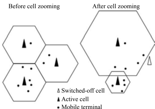
Figure 1: Conceptual scheme of cell zooming.
