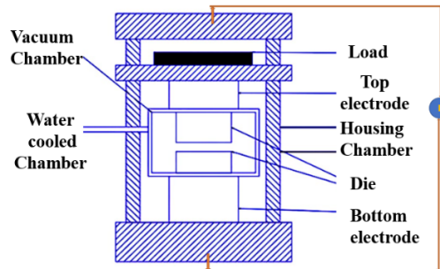
Figure 4: Spark plasma sintering [38].
