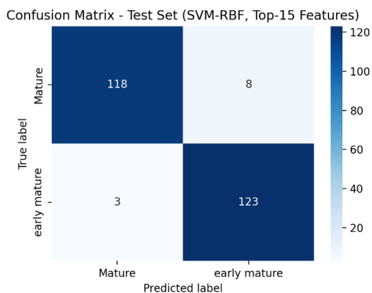
Figure 4 Confusion matrix.
