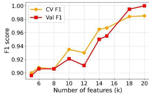
Figure 3 Score vs Number of features ( k ).
