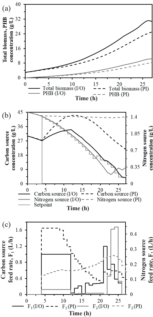
Figure 5: Process response under the regulatory test (a) total biomass and intracellular PHB accumulation (b) carbon and nitrogen source concentration (c) nutrients feed rate.
