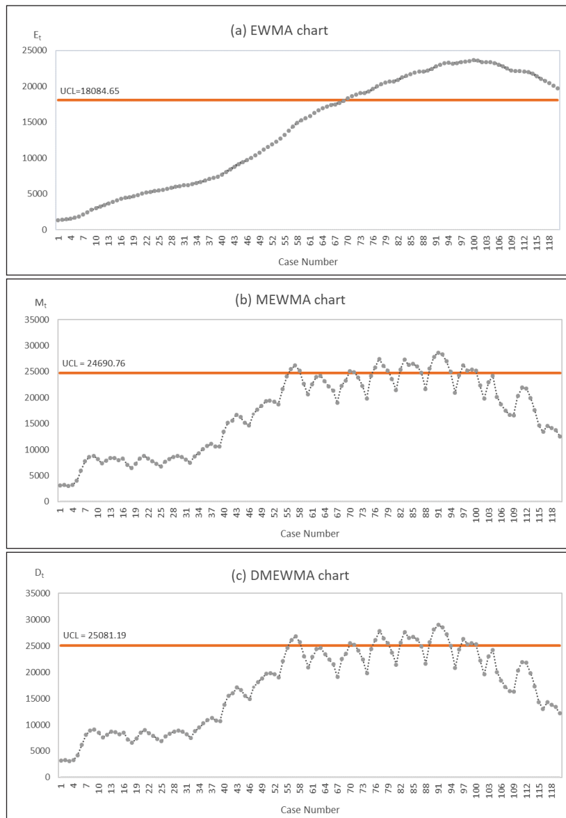
Figure 3: The COVID-19 Thailand dataset fitted to an AR(3) process running on (a) an EWMA chart, (b) a MEWMA chart and (c) a DMEWMA chart.
