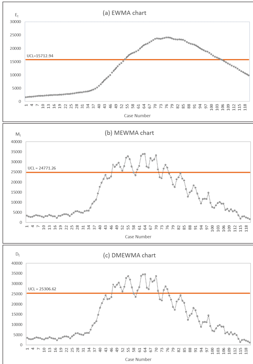
Figure 1: The COVID-19 Malaysia dataset fitted to an AR(1) process running on (a) an EWMA chart, (b) a MEWMA chart and (c) a DMEWMA chart.
