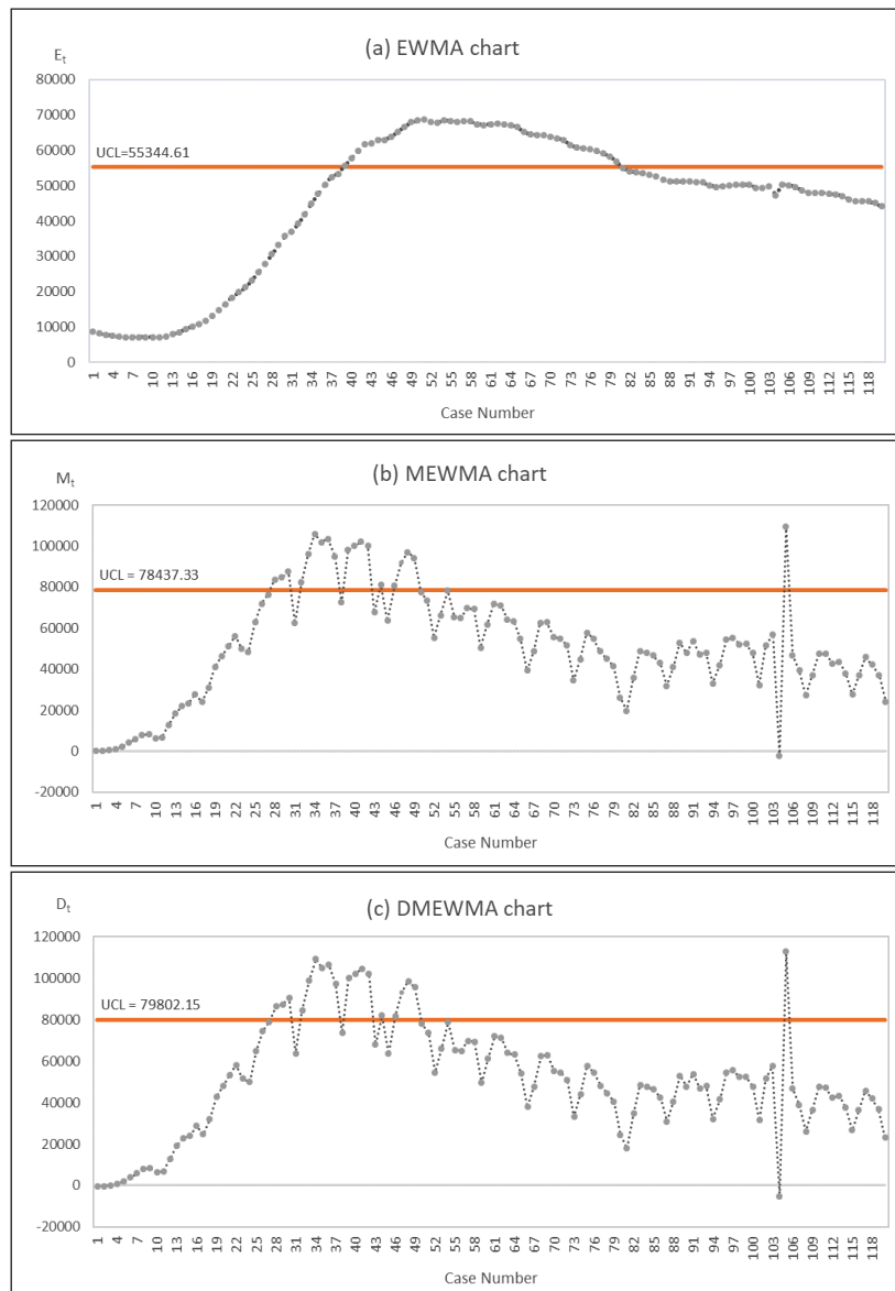
Figure 2: The COVID-19 Japan dataset fitted to an AR(2) process running on (a) an EWMA chart, (b) a MEWMA chart and (c) a DMEWMA chart.
