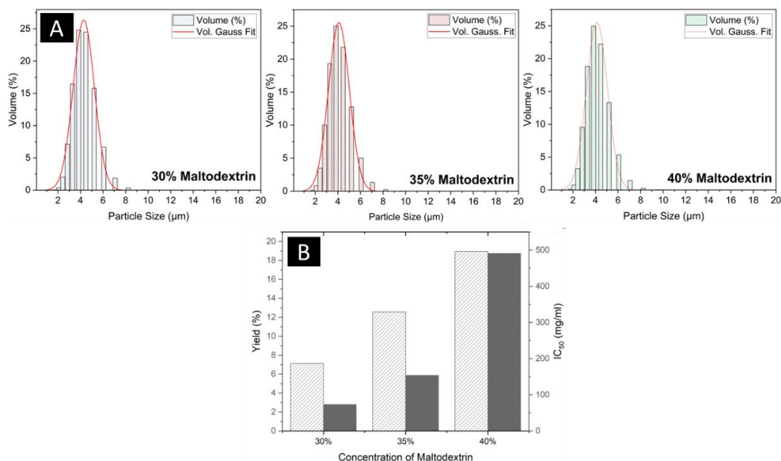
Figure 7. Average particle size (A), yield, and antioxidant activity (B) of the loaded emulsion powder.
