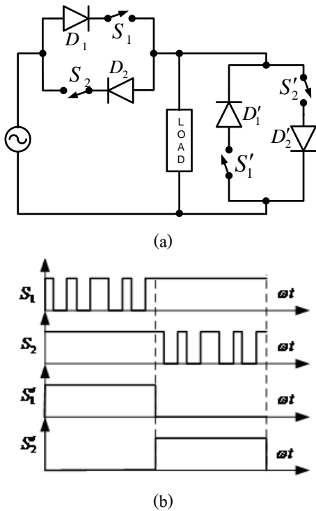
Fig.1 (a) Single-phase PWM AC voltage controlle (b) Conventional fixed-duration PWM Signal
