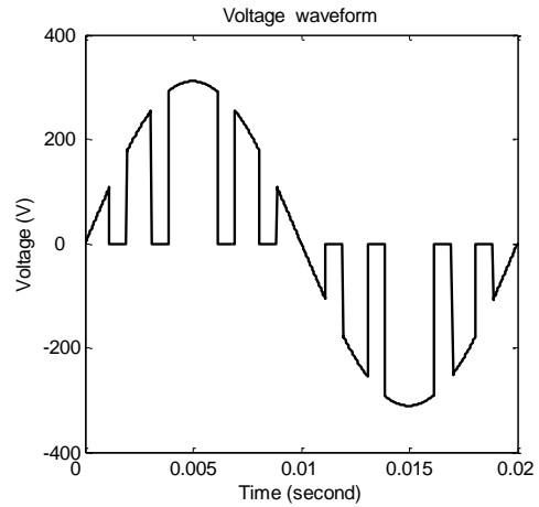
Fig.2 Output waveform of conventional fixed-duration PWM AC voltage controller. The rms voltage of this waveform is 180 V.
