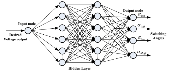
Fig. 5 ANN for optimal switching angles approximation
