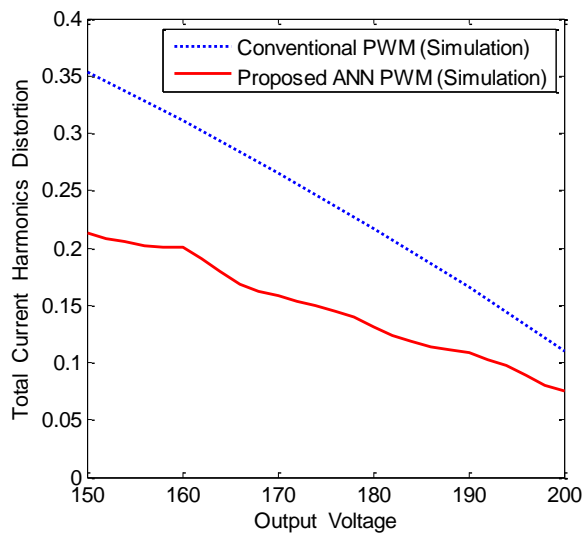
Fig.9 Comparison of THD_i from the proposed technique and the conventional technique PWM for some given desired output voltages\
