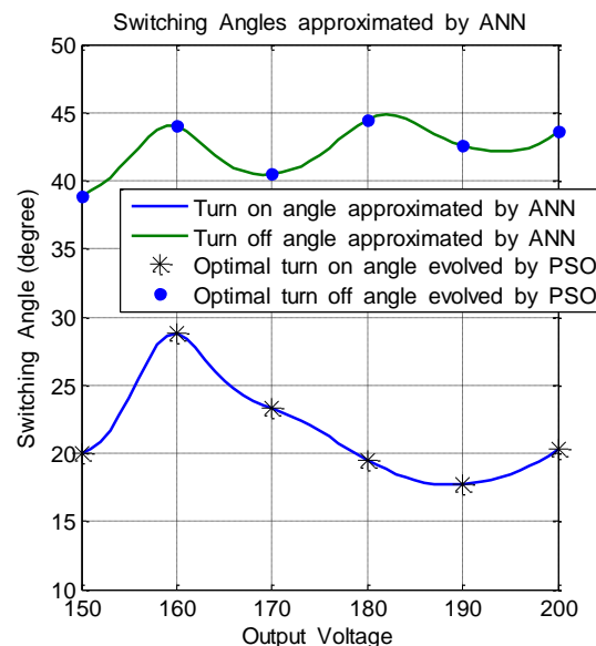
Fig.8 Optimal switching angle versus desired output voltage: Marker '*' and '•' are the optimal angles evolved by PSO that are used for training set. Solid lines are the approximated angles by ANN.
