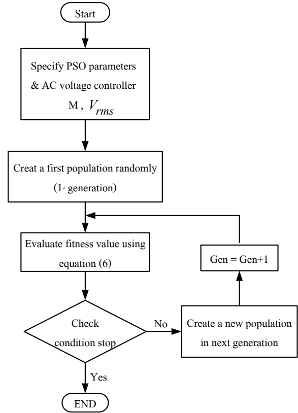
Fig. 4 Flowchart of the proposed design procedure using PSO
